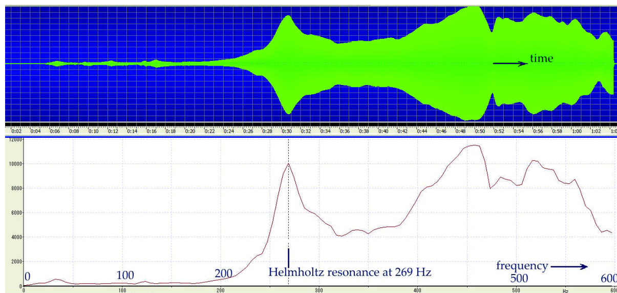
Figure 10: Radiated sound spectrum from a violin excited by sinusoidal vibrations applied to the bridge. Top panel: waveform recorded in GoldWave as frequency is swept in linear ramp. Lower panel: cumulative spectral peak value in WaveSpectra.
