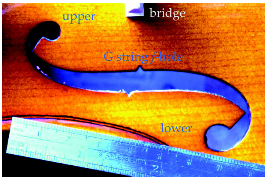
Figure 32: Detail of the f -hole next to the G string of a factory-made violin.
