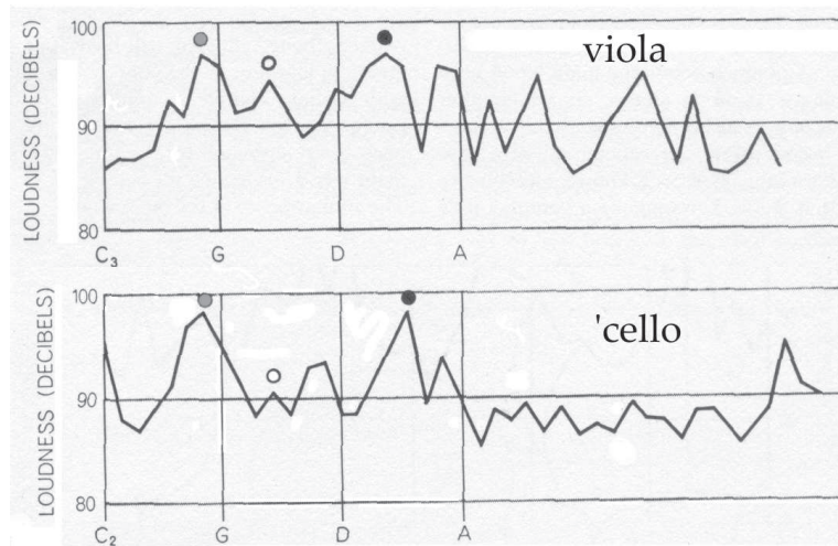
Figure 15: Loudness curves of a viola and a 'cello, after Hutchins
