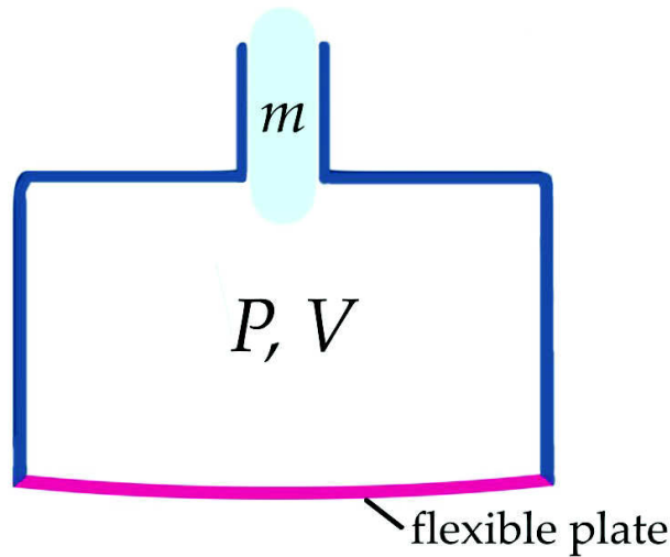
Figure 36: Model of Helmholtz resonator with flexible bottom plate (red).
