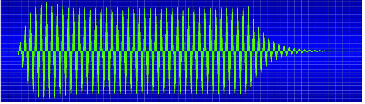
Figure 18: Response of a Helmholtz resonator driven by a tone burst of sine wave just below its resonant frequency.
