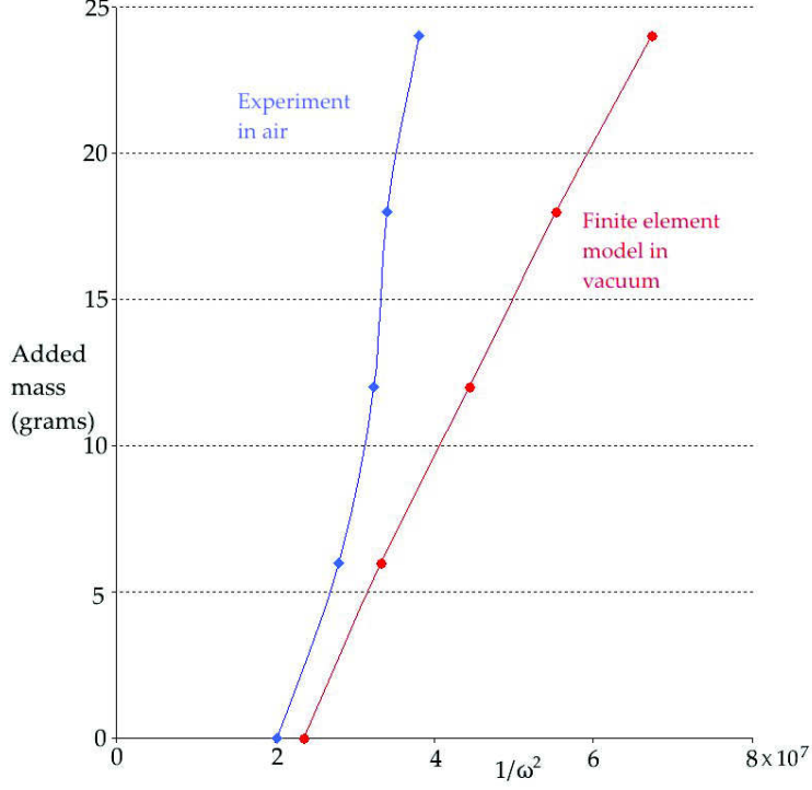
Figure 38: Effect on breathing-mode frequency of adding mass to the back plate of Box C .
