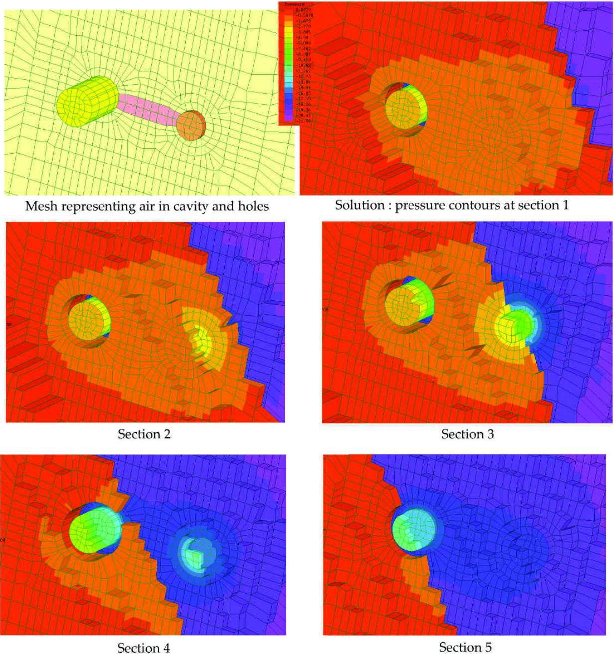
Figure 30: FE modelling of the two holes, one with 19 mm tube attached, joined by a slot. Top left: the FE mesh component representing the air in the aperture and inside the box. Others: contours of acoustic pressure at five adjacent sections through the solution space.
