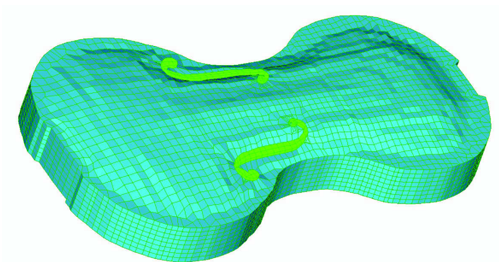
Figure 33: Mesh model of air cavity within a violin, with f -holes.
