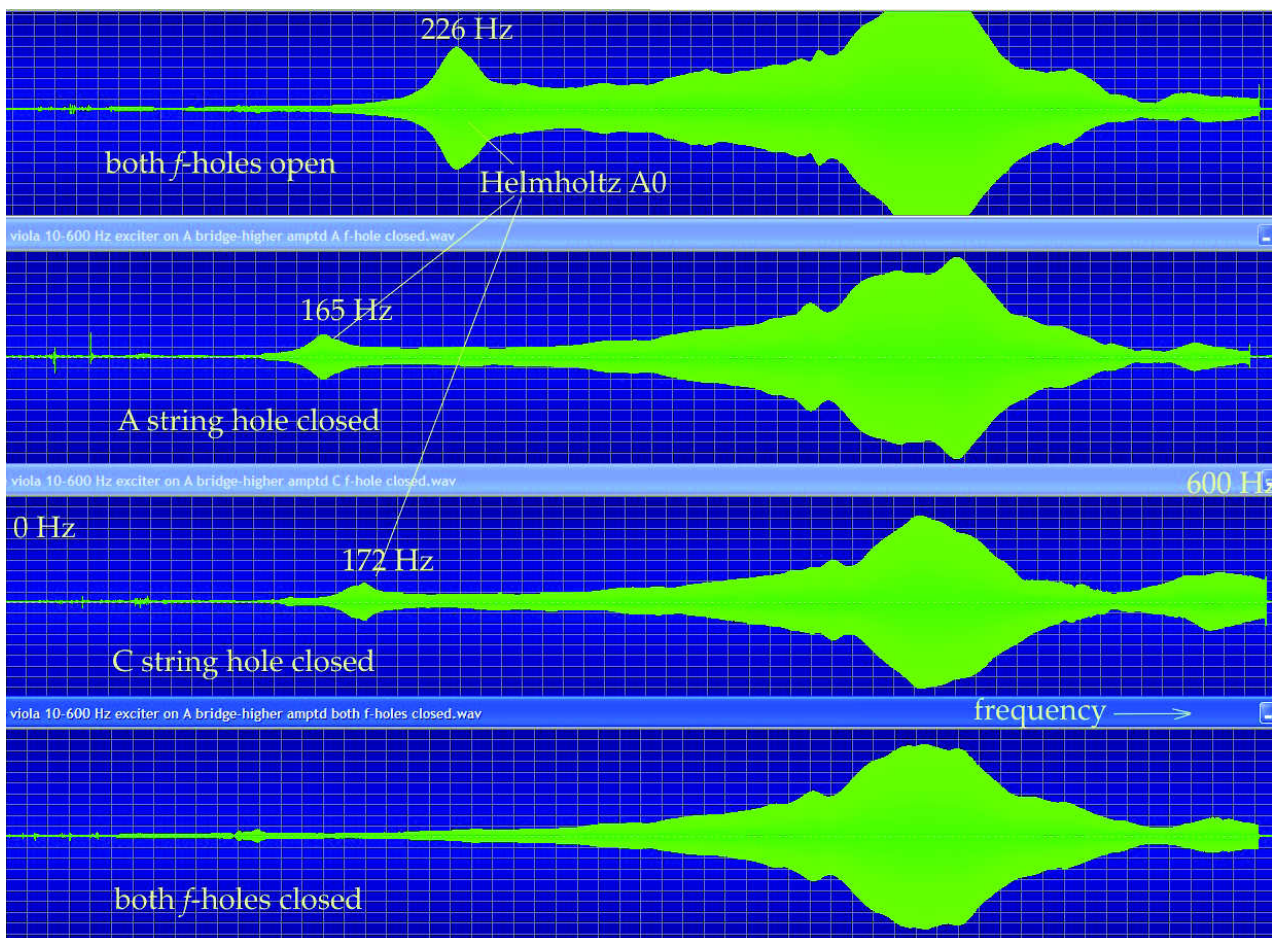
Figure 12: Swept frequency radiated sound from 16\frac{1}{2} inch viola, 0 to 600 Hz, showing effect of closing one or both f -holes.
