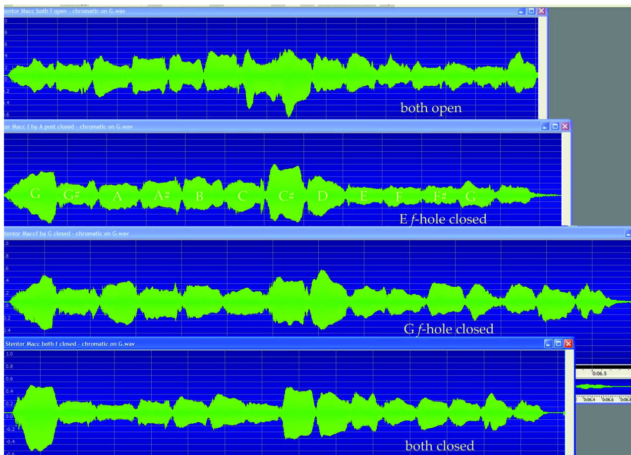
Figure 13: Waveforms as a chromatic scale is played by bowing a violin on the G string under four conditions of the f -holes.
