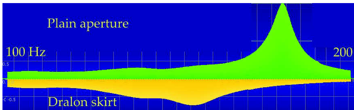
Figure 31: Effect of adding a neck (or skirt) of Dralon cloth (orange inverted spectrum) all around the perimeter of the 61 by 28 mm aperture in Box C. Upper green curve is for the aperture with no Dralon. 100 to 200 Hz.
