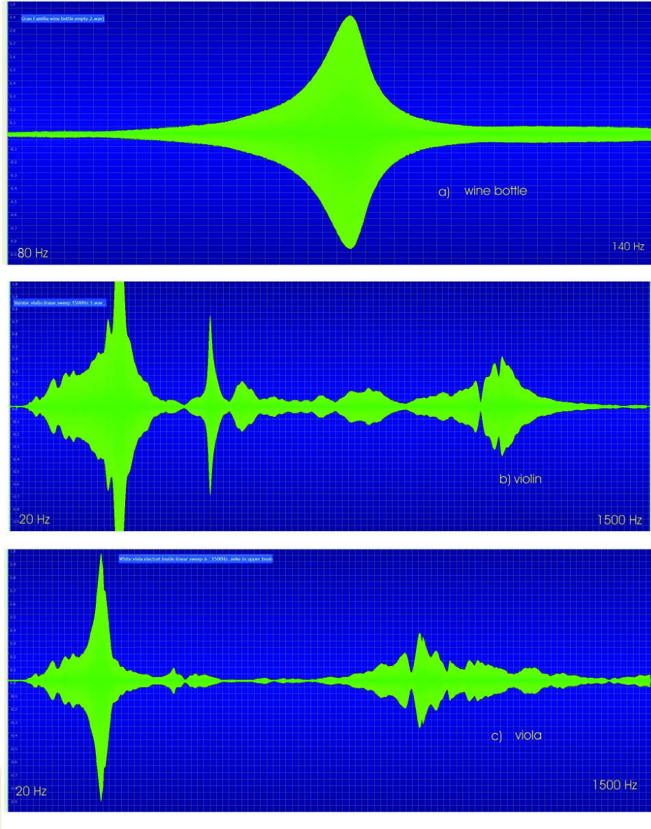
Figure 9: Frequency-amplitude spectra for a) wine bottle, b) violin and c) 16\frac{1}{2} inch viola, recorded with an internal microphone in the arrangement of Figure 6.
