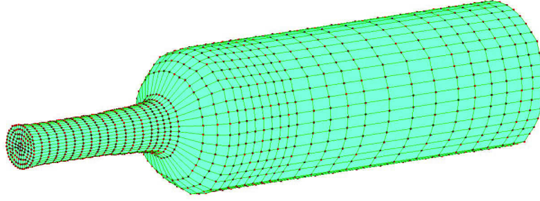
Figure 24: The wine bottle modelled as a finite element mesh.
