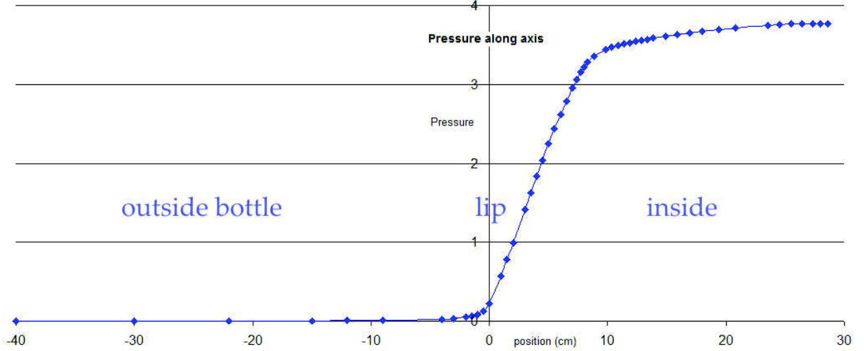
Figure 26: Finite element results for peak acoustic pressure p_a(z) along axis z of empty wine bottle.
