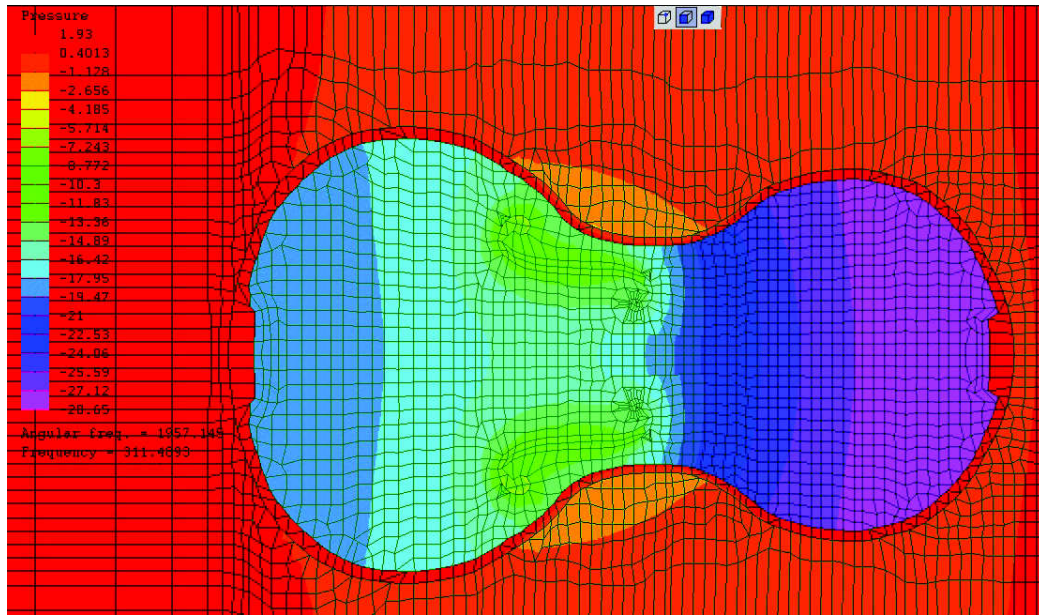
Figure 34: Contours of sound pressure at the A0 Helmholtz resonance at 312 Hz as predicted by LISA. Section through the f -holes.
