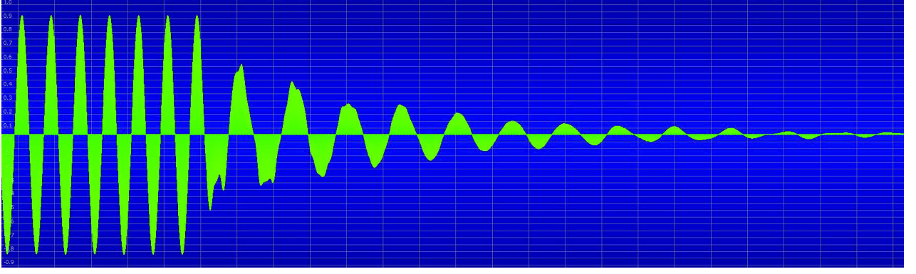
Figure 19: Decay of response after a driving tone burst at about twice the resonant frequency.
