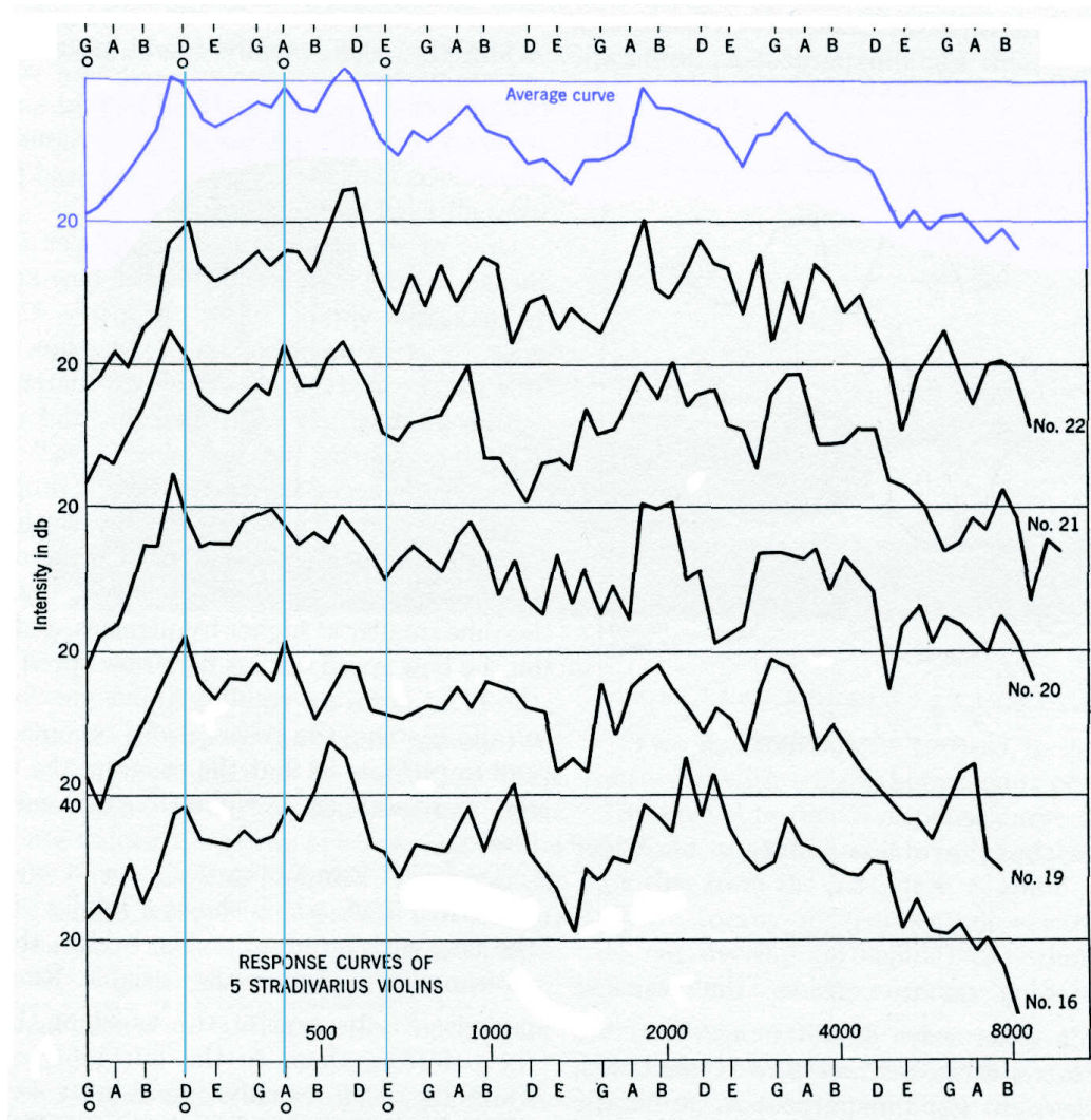
Figure 16: Loudness curves for 5 Stradivarius violins, after Saunders, 1937.
