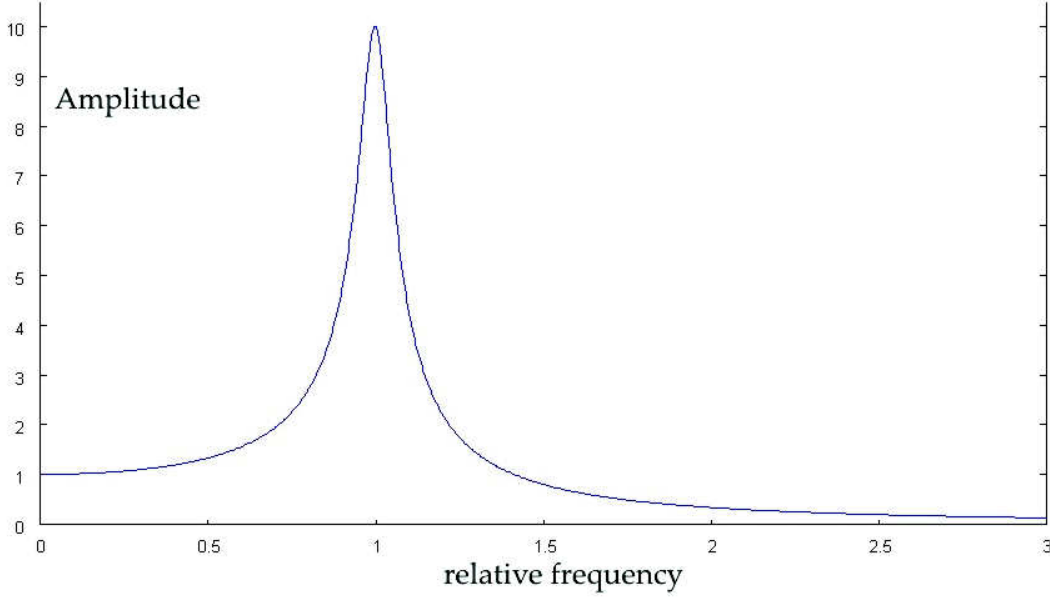
Figure 20: Theoretical frequency response of a damped harmonic oscillator driven at frequency \omega , plotted as function of \omega/\omega_0 . Case M = S = 1 , R = 1/10 .
