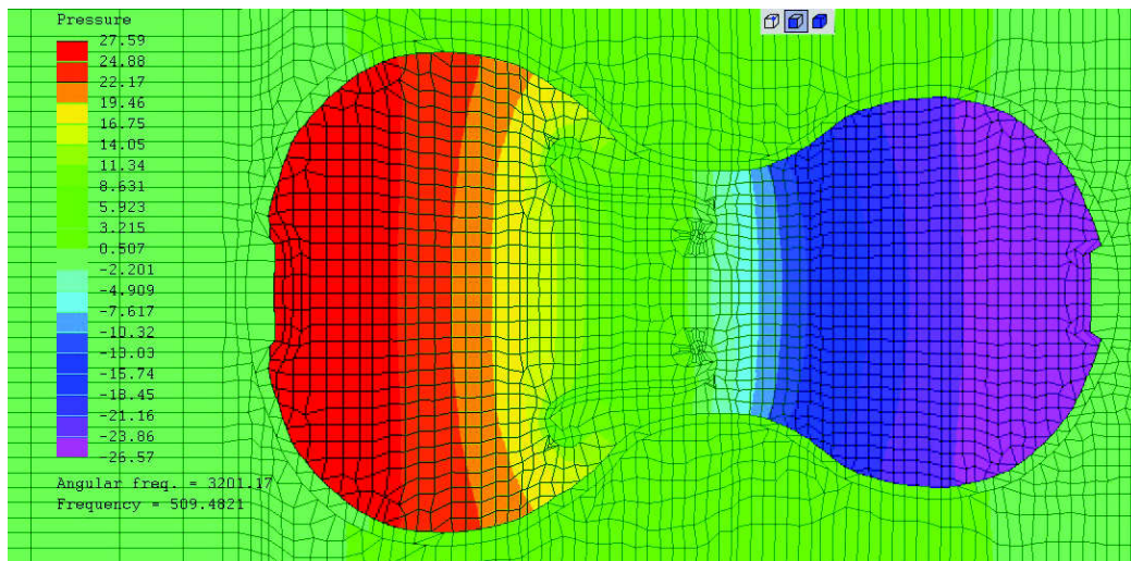
Figure 35: Contours of sound pressure at the A1 resonance at 511 Hz.
