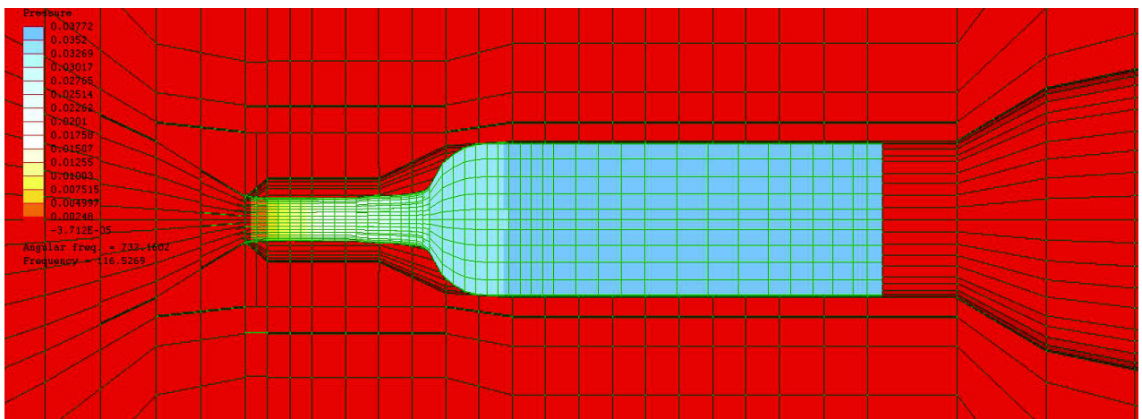
Figure 25: Section through the FE mesh at the Helmholtz resonance of 116.5 \text{ Hz} , showing pressure contours.
