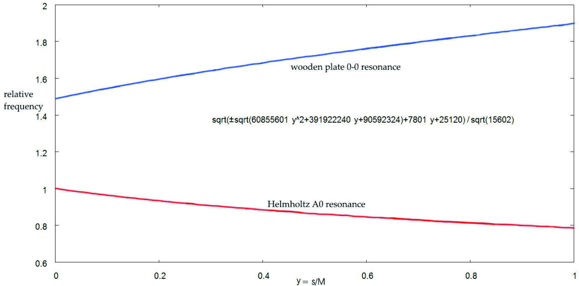
Figure 39: Increase in plate 0-0 modal frequency and decrease in A0 as wood-air coupling s/M increases, normalised to A0=1.
