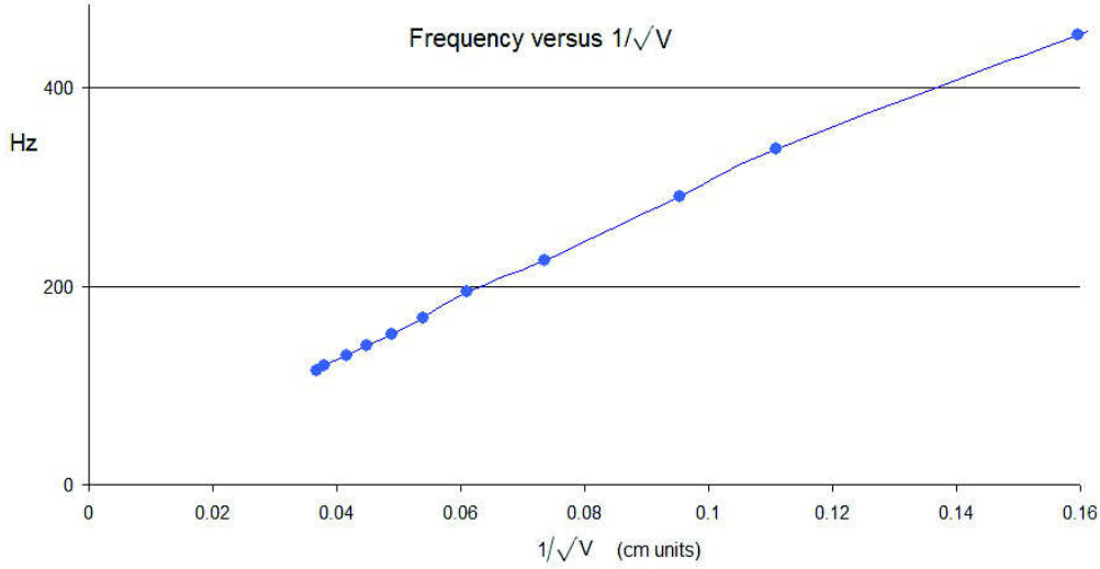
Figure 22: Experimental values of Helmholtz frequency and volume of air in the body of the bottle plotted as f against \frac{1}{\sqrt{V}} .
