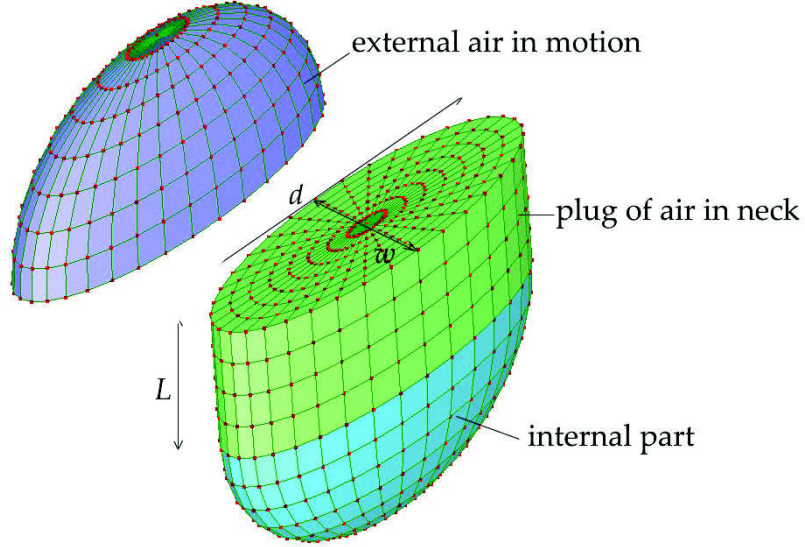
Figure 21: Simple approach to estimating the neck length correction. The shapes represent three volumes of air in vibration at the neck in the cavity. The external cap has been displaced to show the cross section.
