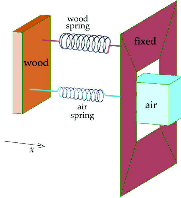
Figure 37: A system with 2 degrees of freedom modelling interaction between air and the box walls.
