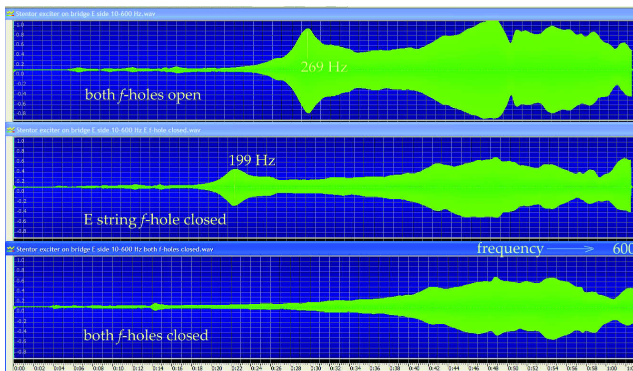
Figure 11: Swept frequency radiated sound of violin, 0 to 600 Hz, with 0, 1 and 2 f -holes closed.
