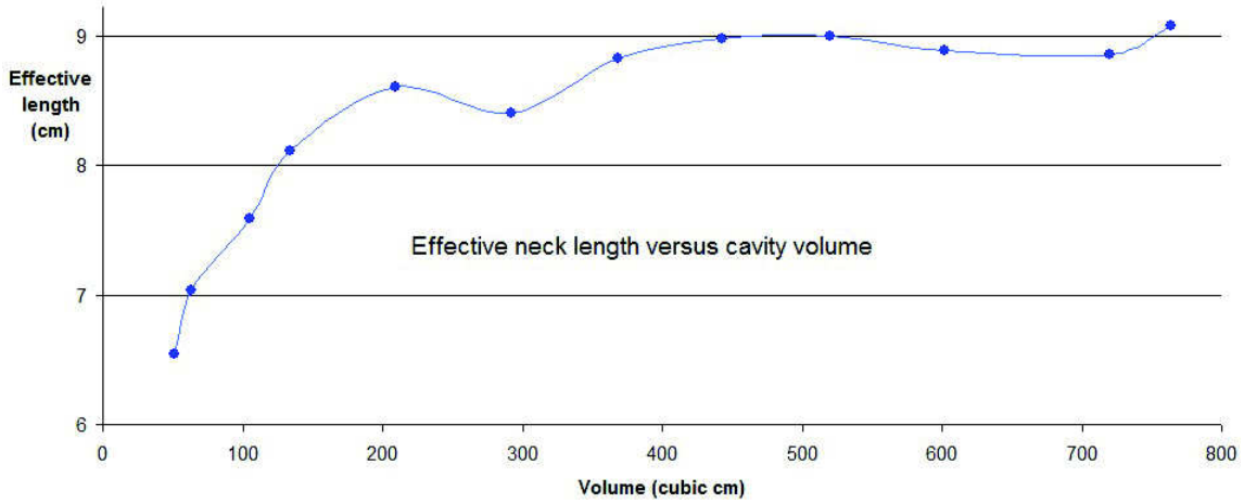
Figure 23: Effective neck length as a function of air volume in the wine bottle.
