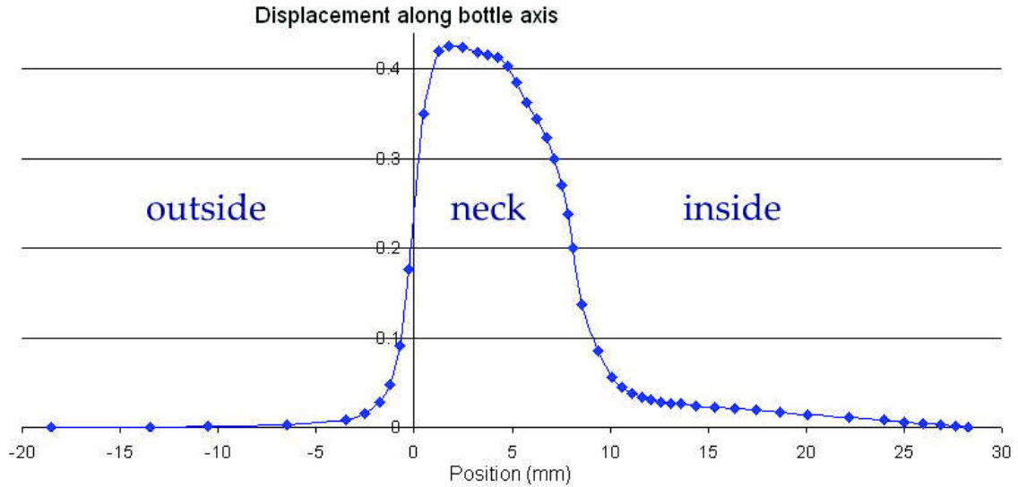
Figure 27: The particle displacement (arbitrary units) along axis z of empty wine bottle showing that almost all movement occurs in the neck.
