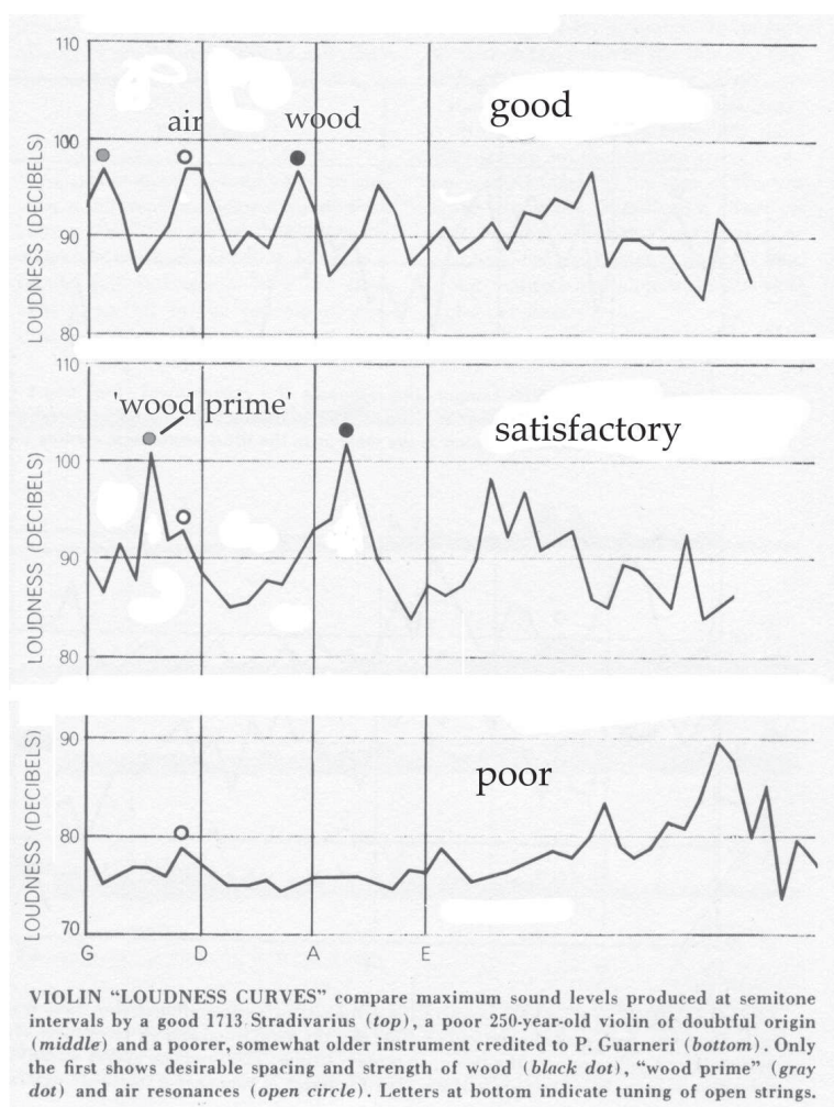
Figure 14: Loudness curves of three violins of different qualities, after Carleen Hutchins.
